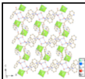
Fig. 2. A packing diagram of the title compound. H atoms are omitted for clarity.
