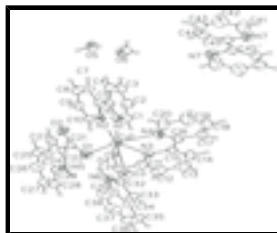
Fig. 1. The molecule structure of the title compound, showing the atom-labelling scheme. Displacement ellipsoids are drawn at the 50% probability level. H atoms are presented as a small spheres of arbitrary radius. Symmetry code: (i) -x, -y + 2, -z + 1 .
